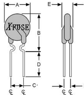
Figure 2 Lead Size: 24AWG Φ 0.51 mm Diameter
